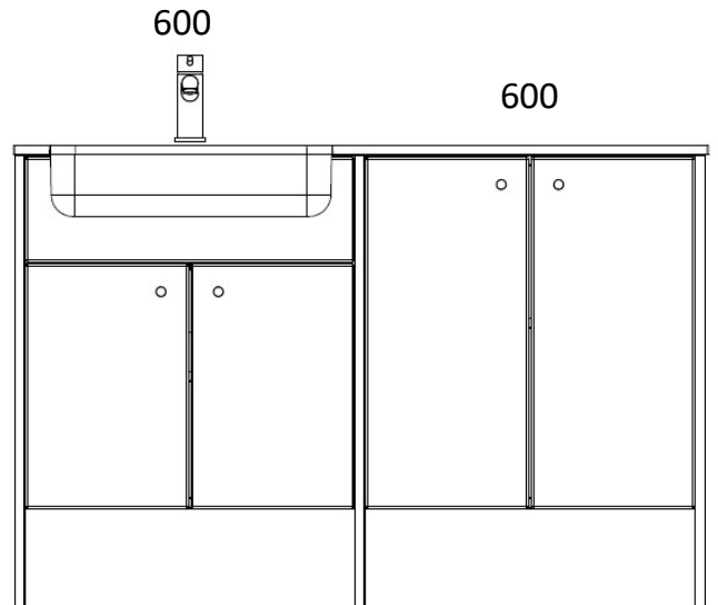
1260 LOMOND 1260 LOMOND BASIN 600 SHORT DOOR BASIN UNIT 600 SHORT DOOR BASE UNIT X3 820 END PANELS X1 PLINTH
