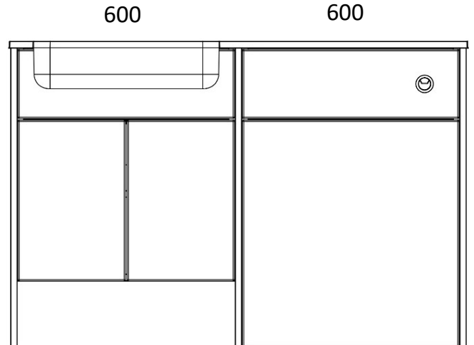
1260 LOMOND BASIN 600 SHORT DOOR BASIN UNIT 600 WC UNIT X3 820 END PANELS X1 PLINTH
