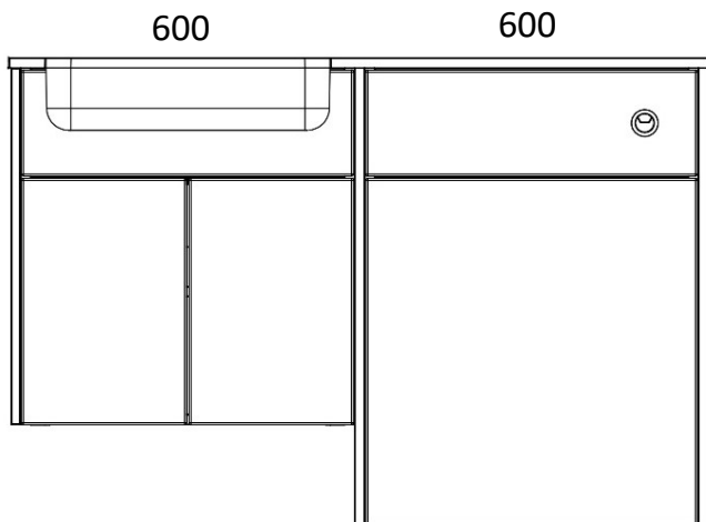
1260 LOMOND 600 SHORT DOOR BASIN UNIT 600 WC UNIT X2 820 END PANELS X1 640 END PANEL
