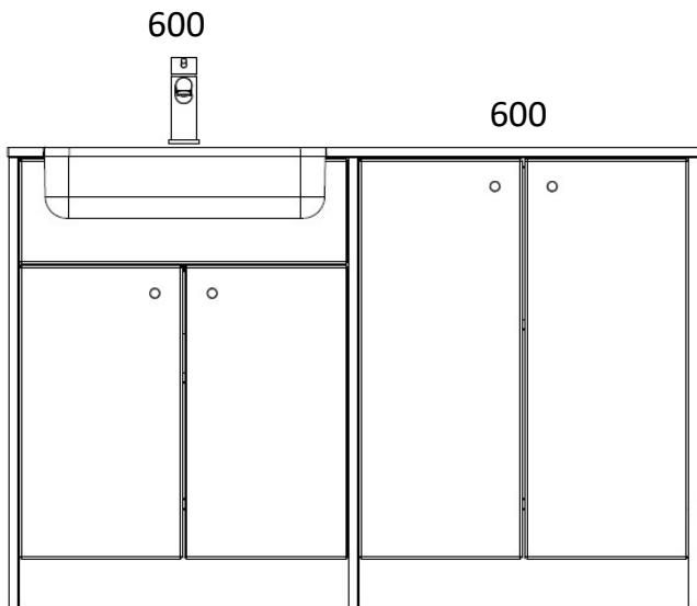
1260 LOMOND 600 LONG DOOR BASIN UNIT 600 LONG BASE UNIT X3 820 END PANELS X1 PLINTH
