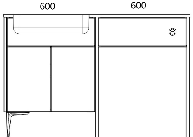
1260 LOMOND 600 SHORT DOOR BASIN UNIT 600 WC UNIT X2 820 END PANELS X1 640 END PANEL X1 DECORATIVE LEG
