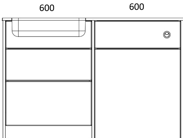
1260 LOMOND 600 LONG DRAWER BASIN UNIT 600 WC UNIT X3 820 END PANELS X1 PLINTH
