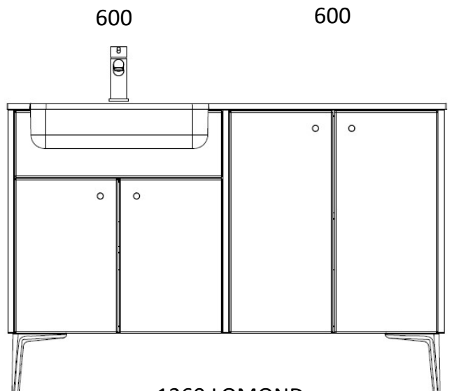
1260 LOMOND 600 SHORT DOOR BASIN UNIT 600 SHORT DOOR BASIN UNIT X3 640 END PANEL X2 DECORATIVE LEG
