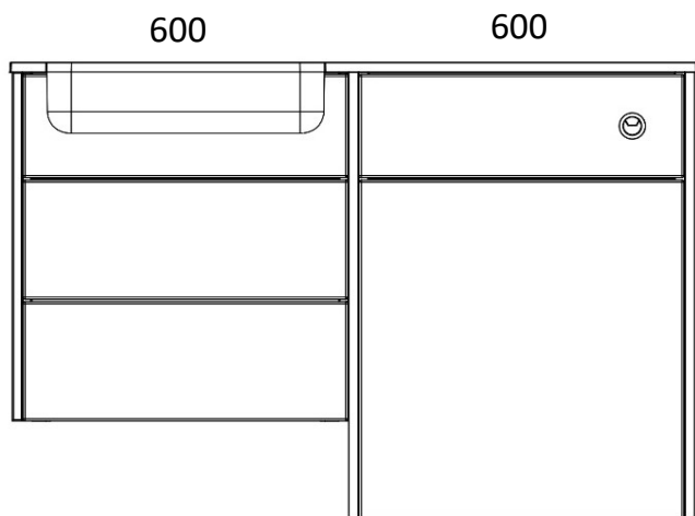
1260 LOMOND 600 SHORT DRAWER BASIN UNIT 600 WC UNIT X2 820 END PANELS X1 640 END PANEL
