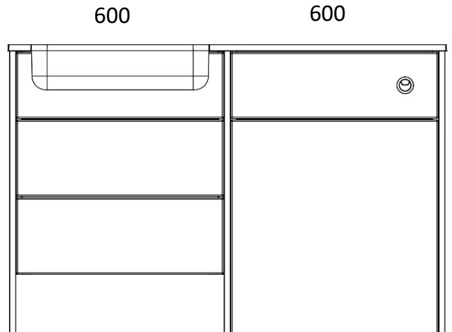
1260 LOMOND 600 SHORT DRAWER BASIN UNIT 600 WC UNIT X3 820 END PANELS X1 PLINTH
