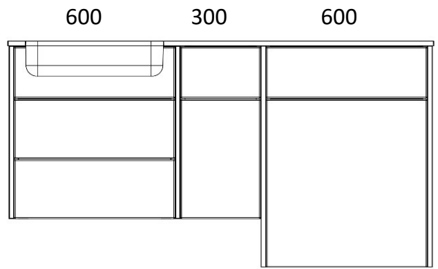
1580 LOMOND 600 SHORT DOOR BASIN UNIT 600 WC UNIT 300 D/LINE BASE UNIT X2 820 END PANELS X2 640 END PANELS
