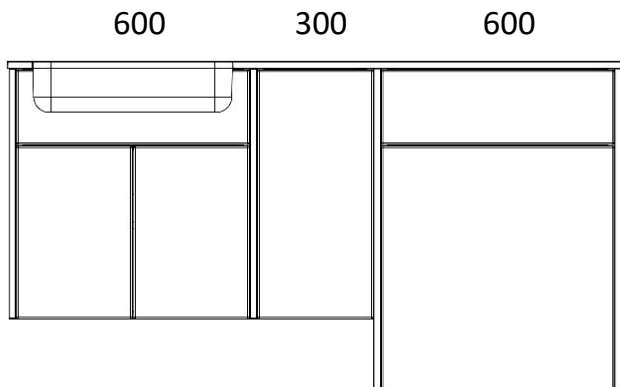
1580 LOMOND 600 SHORT DOOR BASIN UNIT 600 WC UNIT 300 BASE UNIT X2 820 END PANELS X2 640 END PANELS
