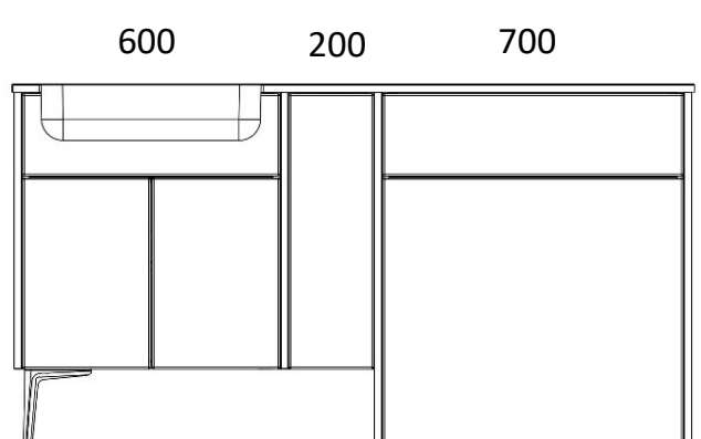
1580 LOMOND 600 SHORT DRAWER BASIN UNIT 700 WC UNIT 200 BASE UNIT X2 820 END PANELS X2 640 END PANEL X1 PLINTH DECORATIVE LEG
