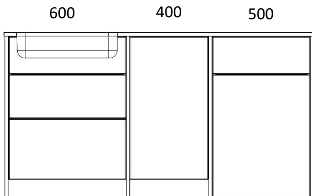
1580 LOMOND 600 LONG DRAWER BASIN UNIT 500 WC UNIT 400 BASE UNIT X4 820 END PANELS X1 PLINTH
