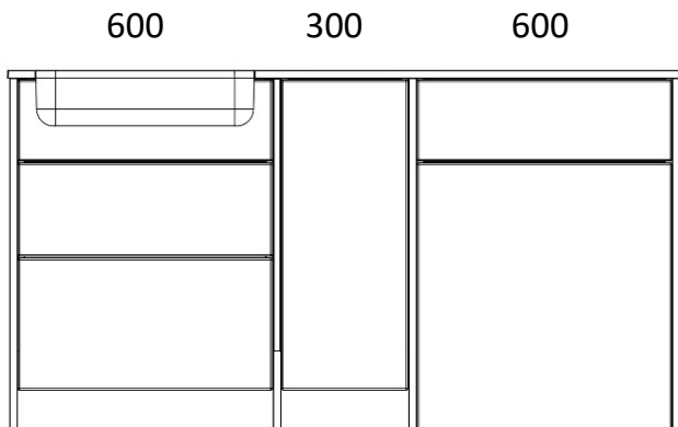
1580 LOMOND 600 LONG DRAWER BASIN UNIT 600 WC UNIT 300 BASE UNIT LONG DOORS X4 820 END PANELS X1 PLINTH
