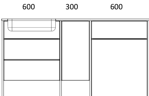
1580 LOMOND 600 SHORT DRAWER BASIN UNIT 600 WC UNIT 300 BASE UNIT SHORT DOORS X4 820 END PANELS
