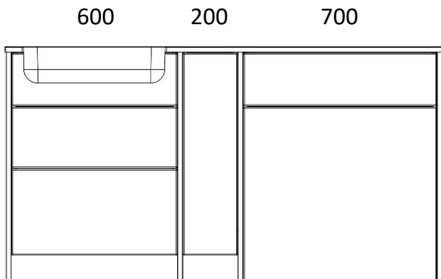
1580 LOMOND 600 LONG DOOR BASIN UNIT 700 WC UNIT 200 BASE UNIT X4 820 END PANELS
