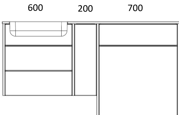
1580 LOMOND 600 SHORT DRAWER BASIN UNIT 700 WC UNIT 200 BASE UNIT X2 820 END PANELS X2 640 END PANEL X1 PLINTH
