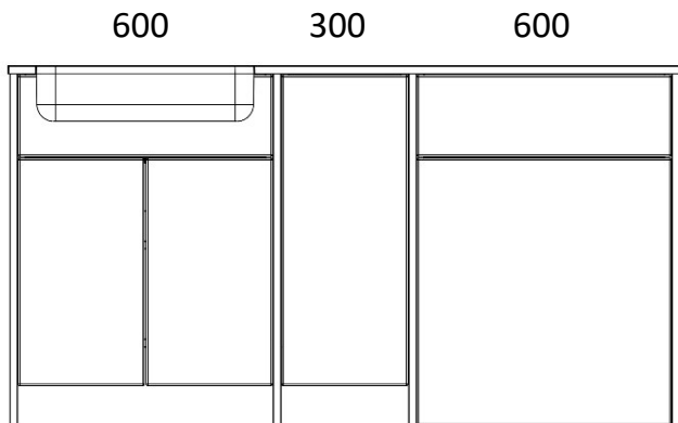
1580 LOMOND 600 LONG DOOR BASIN UNIT 600 WC UNIT 300 BASE UNIT LONG DOORS X4 820 END PANELS X1 PLINTH
