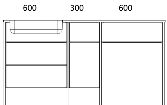
1580 LOMOND 600 SHORT DRAWER BASIN UNIT 600 WC UNIT 300 D/LINE BASE UNIT SHORT DOORS X4 820 END PANELS
