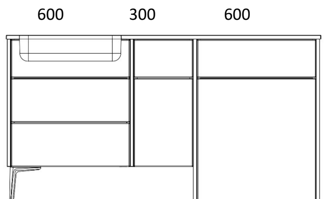
1580 LOMOND 600 SHORT DOOR BASIN UNIT 600 WC UNIT 300 D/LINE BASE UNIT X2 820 END PANELS X2 640 END PANELS DECORATIVE LEG
