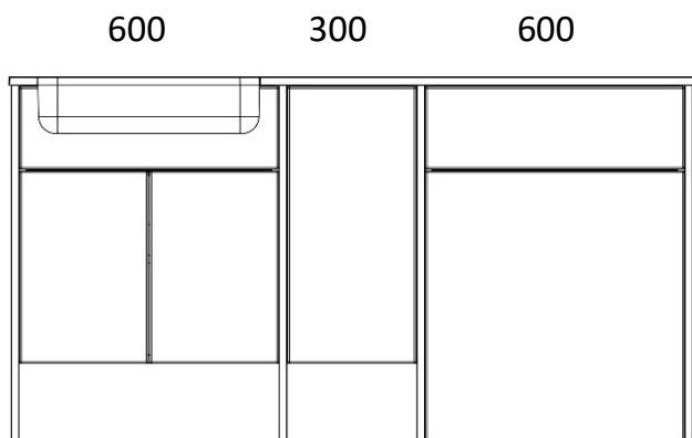
1580 LOMOND 600 SHORT DOOR BASIN UNIT 600 WC UNIT 300 BASE UNIT SHORT DOORS X4 820 END PANELS
