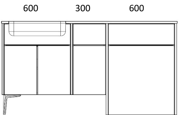
1580 LOMOND 600 SHORT DOOR BASIN UNIT 600 WC UNIT 300 D/LINE BASE UNIT X2 820 END PANELS X2 640 END PANELS DECORATIVE LEG
