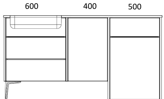
1580 LOMOND 600 SHORT DOOR BASIN UNIT 600 WC UNIT 400 BASE UNIT X2 820 END PANELS X2 640 END PANELS DECORATIVE LEG
