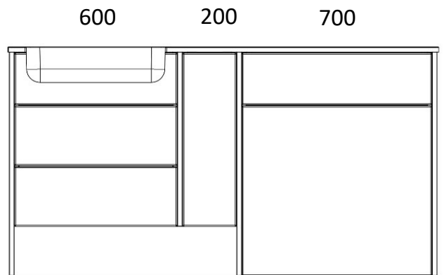
1580 LOMOND 600 SHORT DRAWER BASIN UNIT 700 WC UNIT 200 BASE UNIT X3 820 END PANELS X1 640 END PANEL X1 PLINTH
