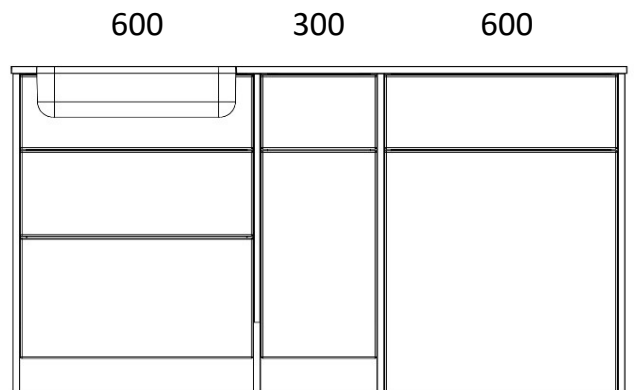
1580 LOMOND 600 LONG DRAWER BASIN UNIT 600 WC UNIT 300 D/LINE BASE UNIT LONG DOORS X4 820 END PANELS X1 PLINTH
