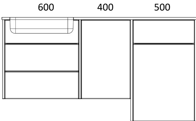
1580 LOMOND 600 SHORT DOOR BASIN UNIT 500 WC UNIT 400 BASE UNIT X2 820 END PANELS X2 640 END PANELS
