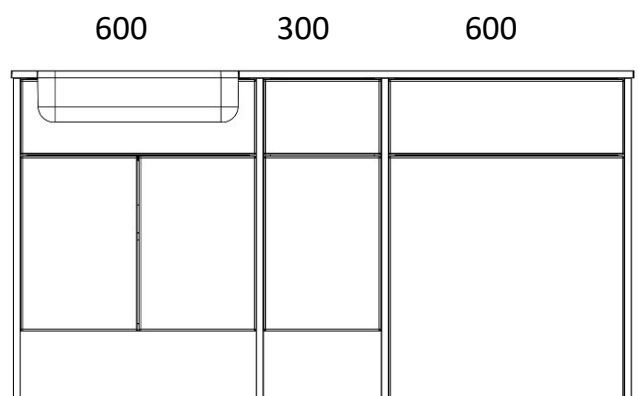
1580 LOMOND 600 SHORT DOOR BASIN UNIT 600 WC UNIT 300 D/LINE BASE UNIT SHORT DOORS X4 820 END PANELS
