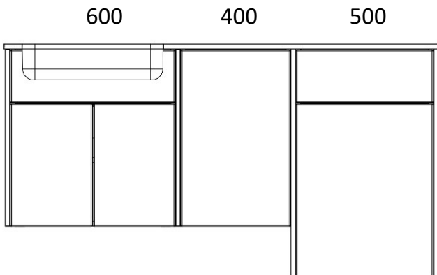
1580 LOMOND 600 SHORT DOOR BASIN UNIT 500 WC UNIT 400 BASE UNIT X2 820 END PANELS X2 640 END PANELS
