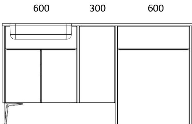
1580 LOMOND 600 SHORT DOOR BASIN UNIT 600 WC UNIT 300 BASE UNIT X2 820 END PANELS X2 640 END PANELS DECORATIVE LEG
