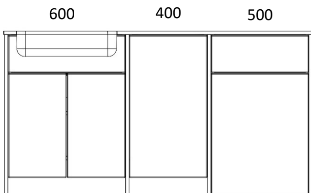
1580 LOMOND 600 SHORT DOOR BASIN UNIT 500 WC UNIT 400 BASE UNIT X4 820 END PANELS X1 PLINTH
