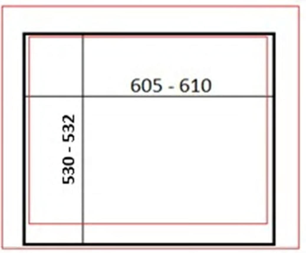
Critical Slip Set Inner Dimensions
